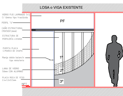
Detalle Panel T4
