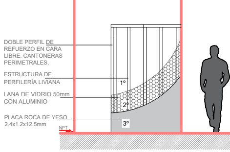
Detalle Panel T1
