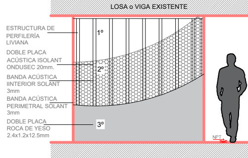
Detalle Panel T5
