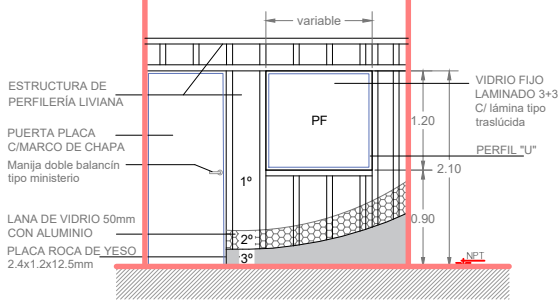
Detalle Panel T3
