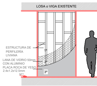
Detalle Panel T2
