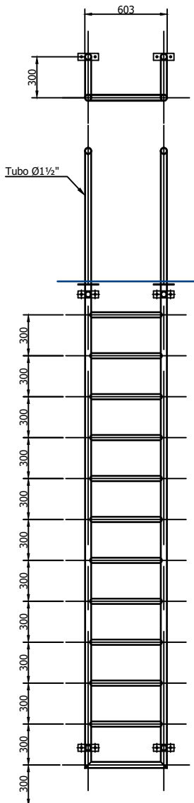
VISTA FRONTAL
