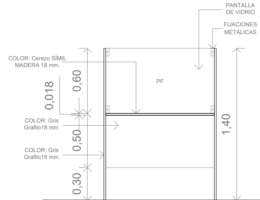
Vista Frontal
